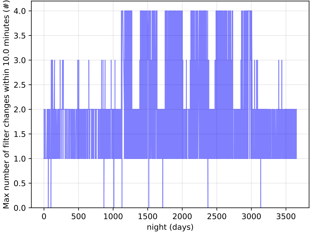
telescope_jerk_v3.5_10yrs Per Night: Max number of filter changes within 10.0 minutes
