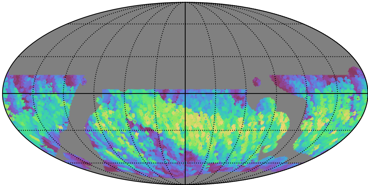
telescope_jerk_v3.5_10yrs WFD z band: Max normairmass
