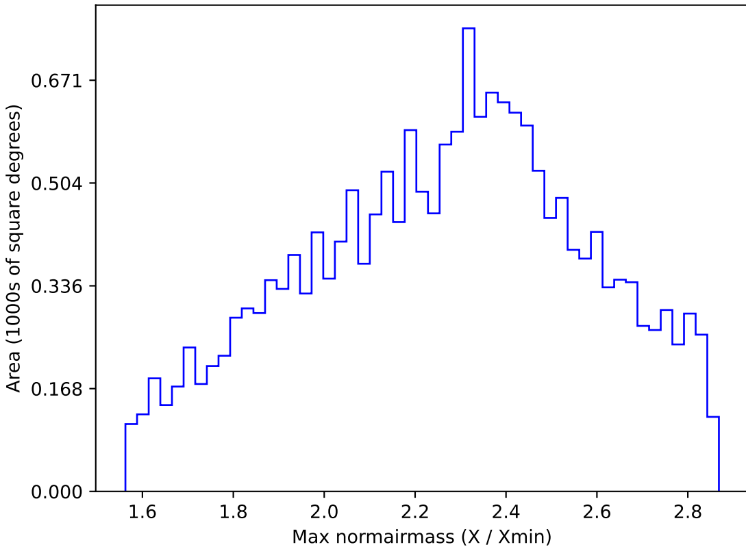
telescope_jerk_v3.5_10yrs WFD z band: Max normairmass
