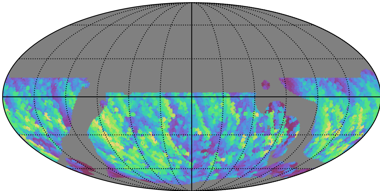
telescope_jerk_v3.5_10yrs WFD y band: Max normairmass
