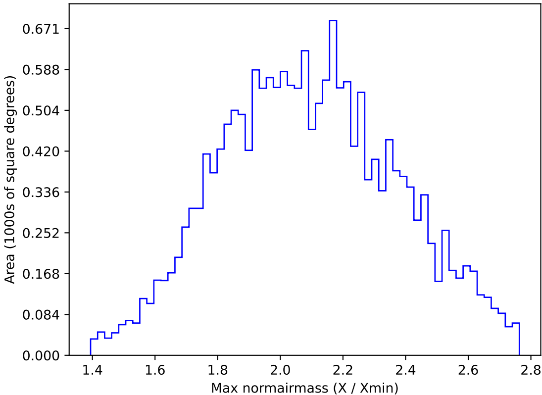
telescope_jerk_v3.5_10yrs WFD y band: Max normairmass
