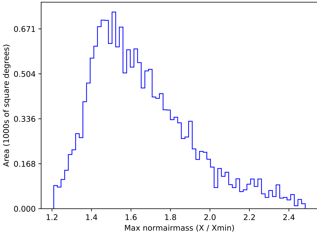
telescope_jerk_v3.5_10yrs WFD u band: Max normairmass
