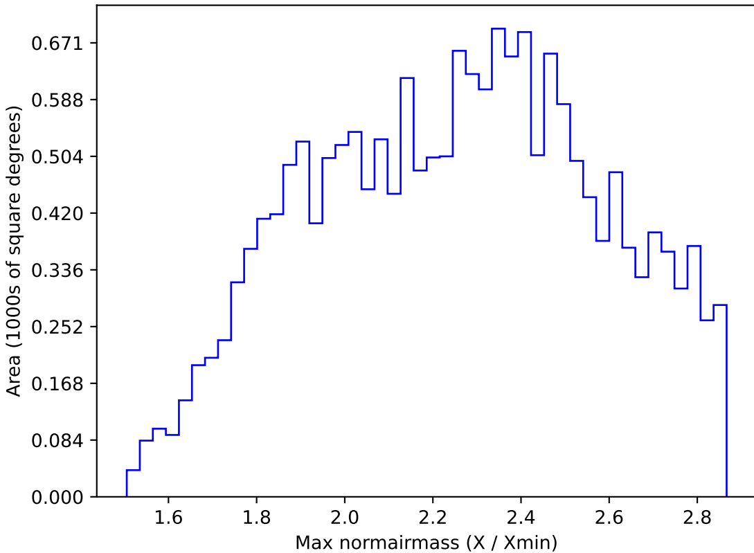
telescope_jerk_v3.5_10yrs WFD i band: Max normairmass
