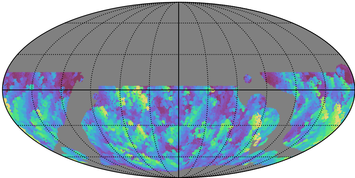
telescope_jerk_v3.5_10yrs WFD g band: Max normairmass
