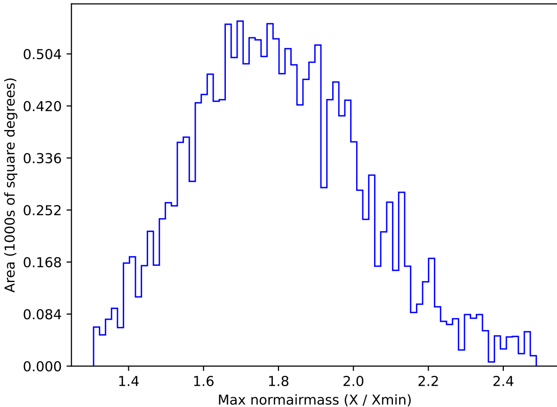
telescope_jerk_v3.5_10yrs WFD g band: Max normairmass
