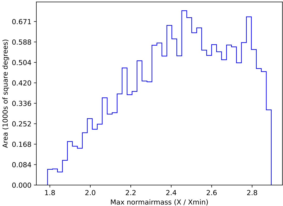
telescope_jerk_v3.5_10yrs WFD all bands: Max normairmass
