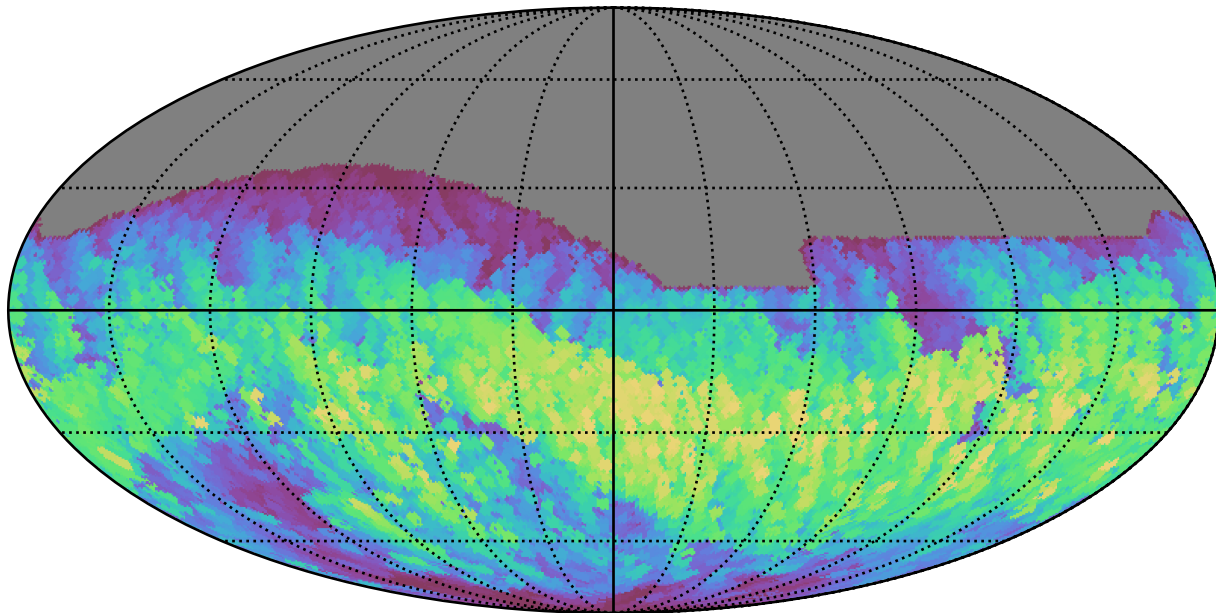
telescope_jerk_v3.5_10yrs All sky z band: Max normairmass
