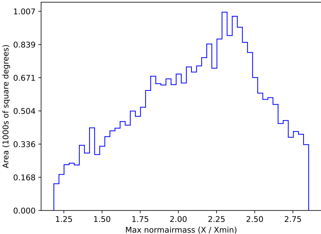
telescope_jerk_v3.5_10yrs All sky z band: Max normairmass
