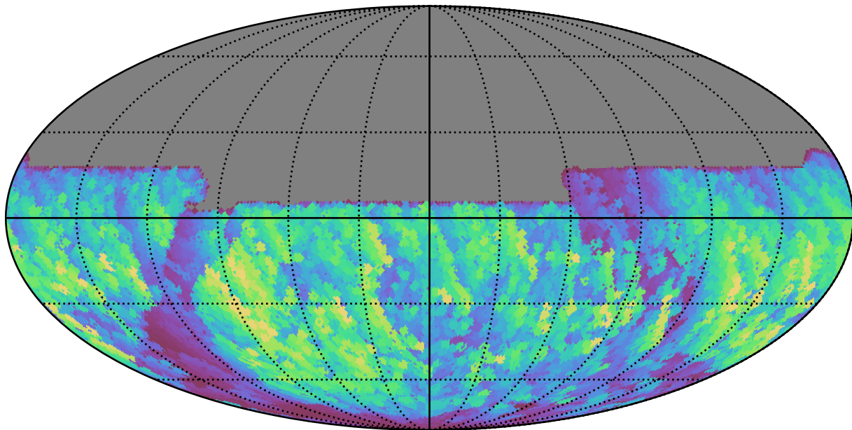
telescope_jerk_v3.5_10yrs All sky y band: Max normairmass
