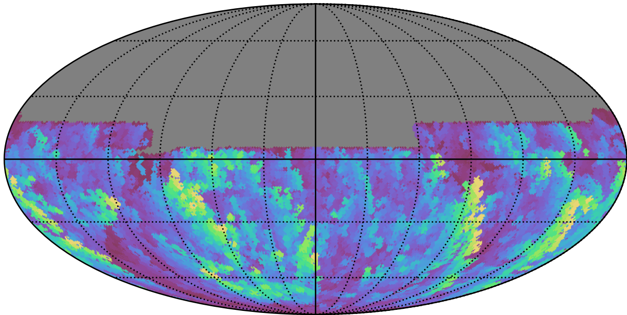
telescope_jerk_v3.5_10yrs All sky u band: Max normairmass
