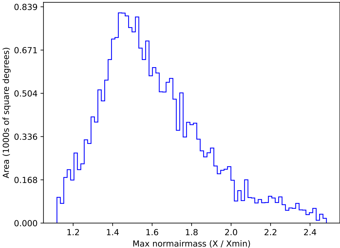
telescope_jerk_v3.5_10yrs All sky u band: Max normairmass
