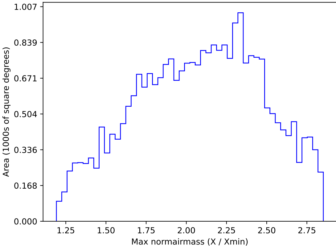
telescope_jerk_v3.5_10yrs All sky r band: Max normairmass
