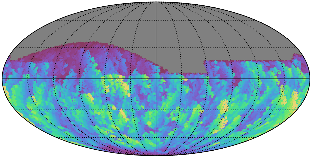
telescope_jerk_v3.5_10yrs All sky g band: Max normairmass
