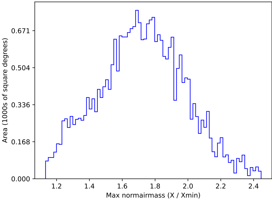
telescope_jerk_v3.5_10yrs All sky g band: Max normairmass
