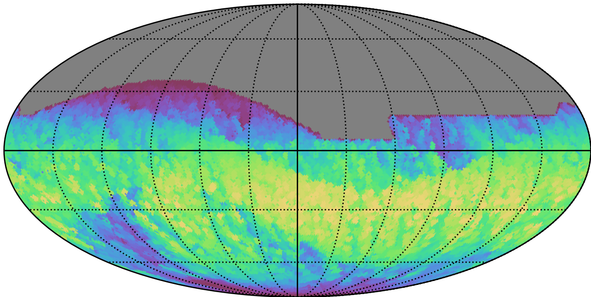
telescope_jerk_v3.5_10yrs All sky all bands: Max normairmass
