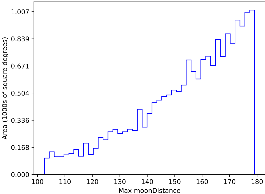
telescope_jerk_v3.5_10yrs WFD z band: Max moonDistance
