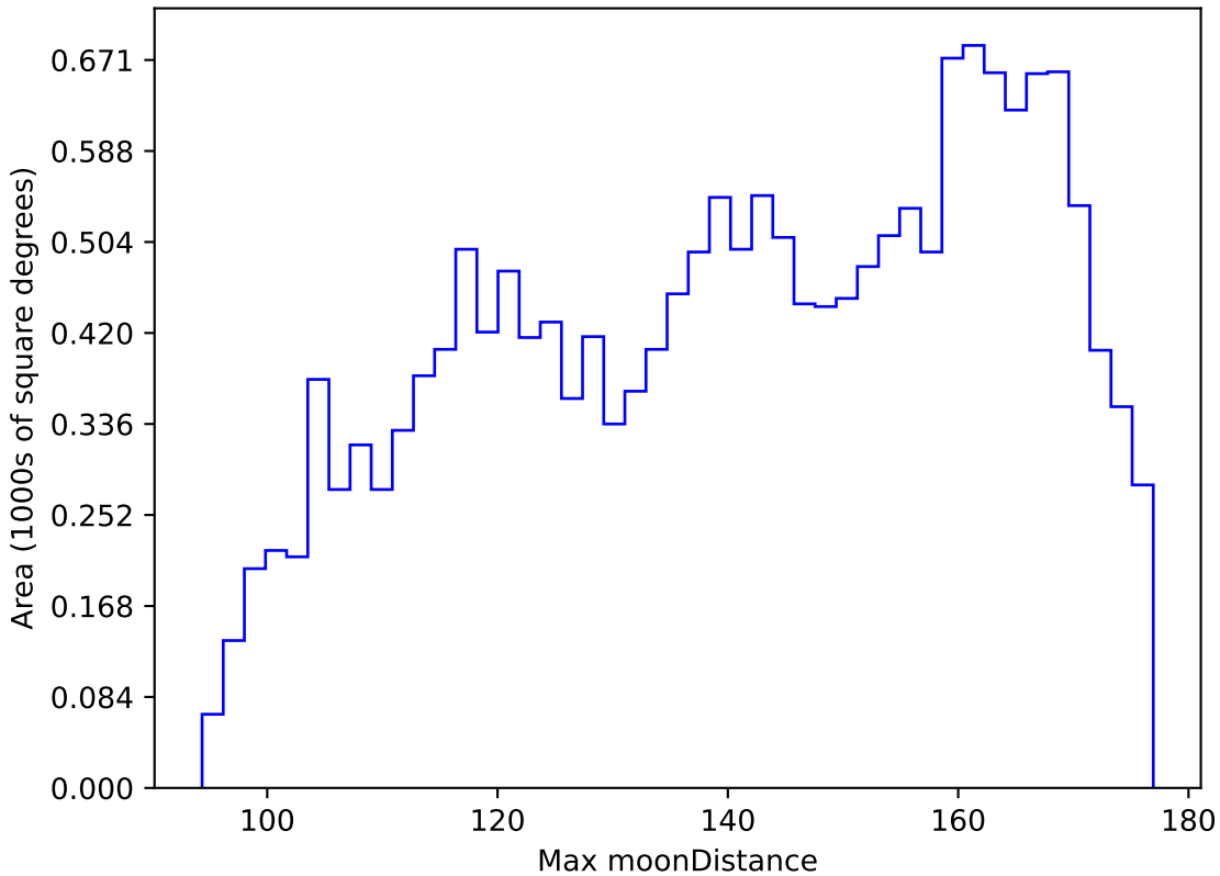
telescope_jerk_v3.5_10yrs WFD y band: Max moonDistance
