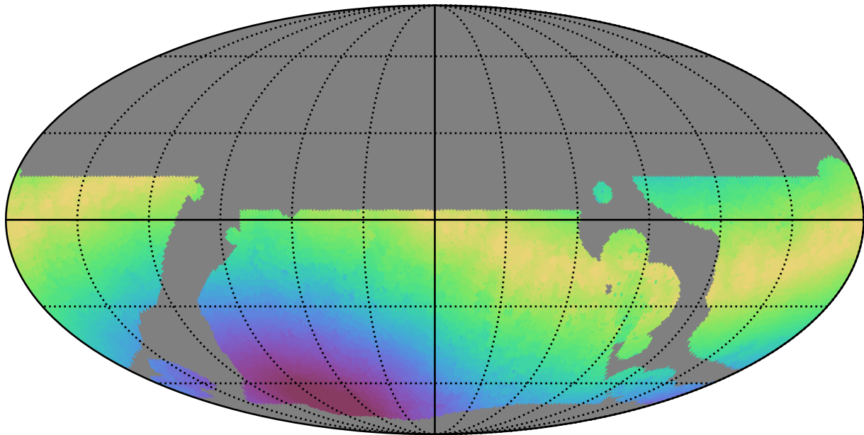
telescope_jerk_v3.5_10yrs WFD u band: Max moonDistance
