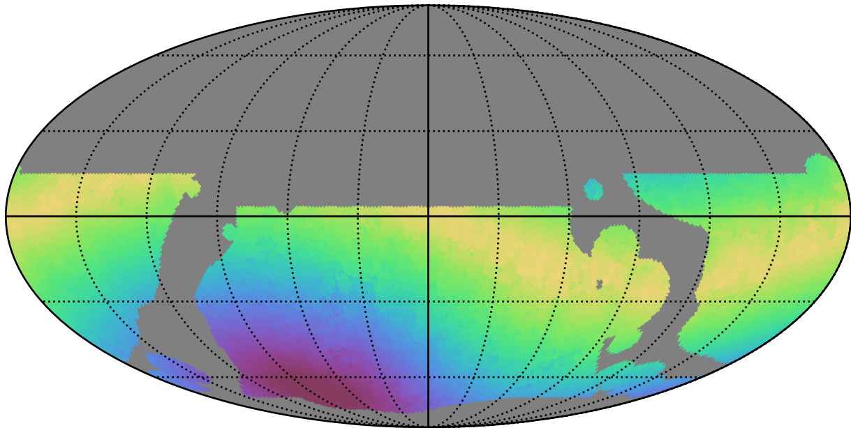
telescope_jerk_v3.5_10yrs WFD i band: Max moonDistance
