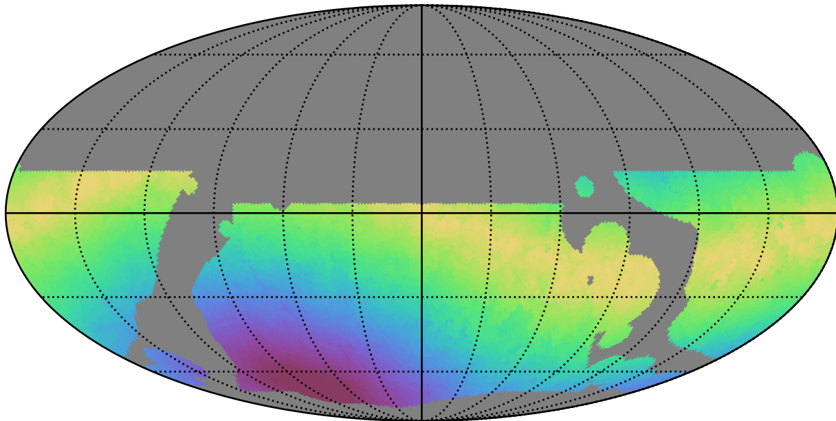
telescope_jerk_v3.5_10yrs WFD g band: Max moonDistance
