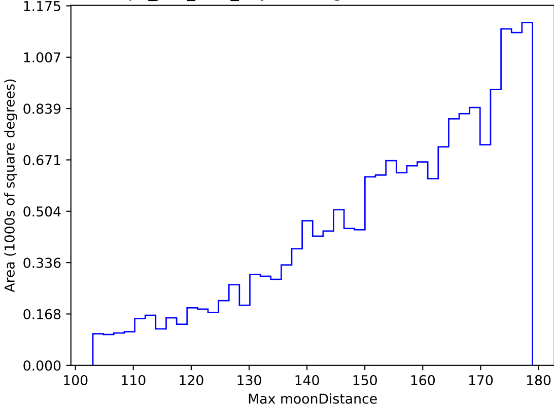
telescope_jerk_v3.5_10yrs WFD g band: Max moonDistance
