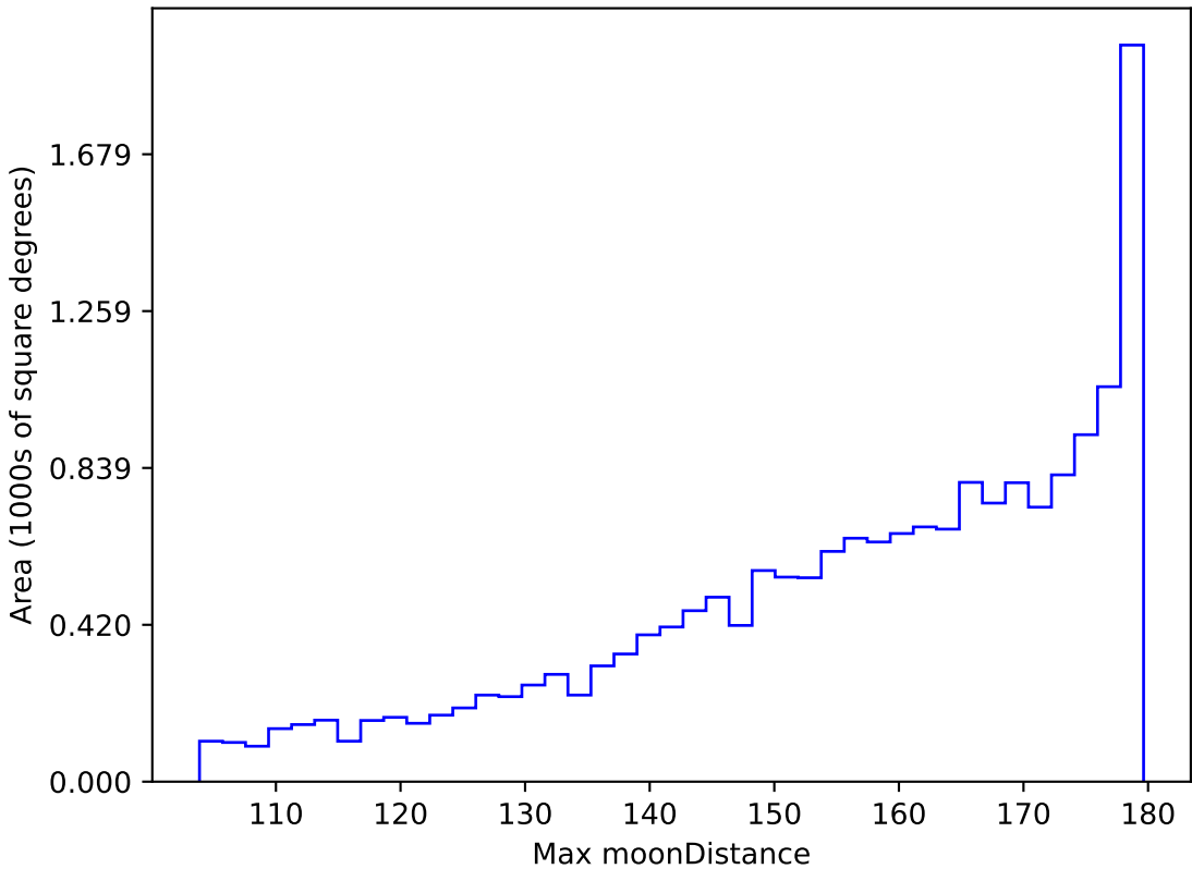
telescope_jerk_v3.5_10yrs WFD all bands: Max moonDistance
