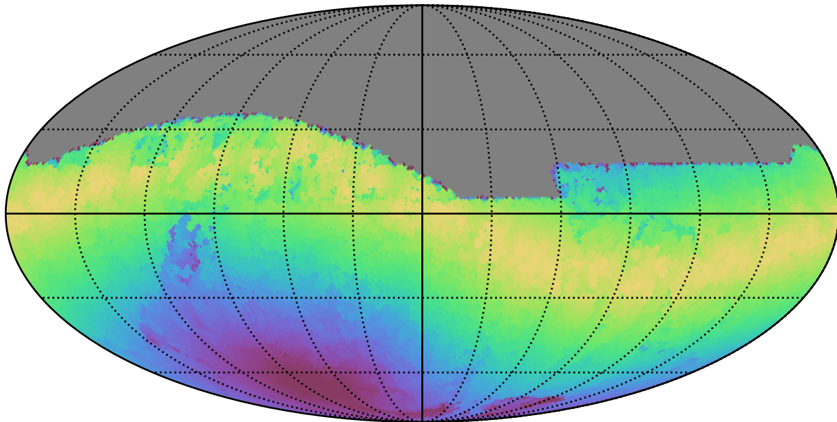
telescope_jerk_v3.5_10yrs All sky z band: Max moonDistance
