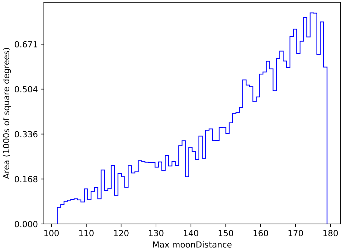
telescope_jerk_v3.5_10yrs All sky z band: Max moonDistance
