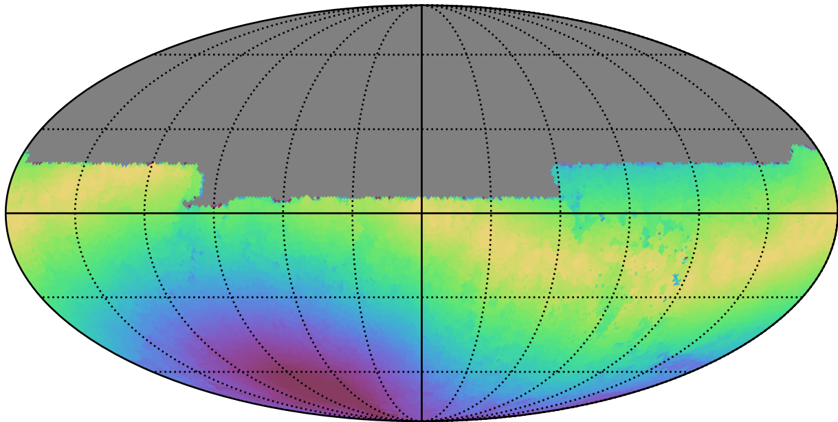
telescope_jerk_v3.5_10yrs All sky u band: Max moonDistance
