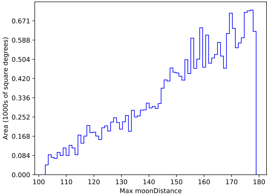
telescope_jerk_v3.5_10yrs All sky u band: Max moonDistance
