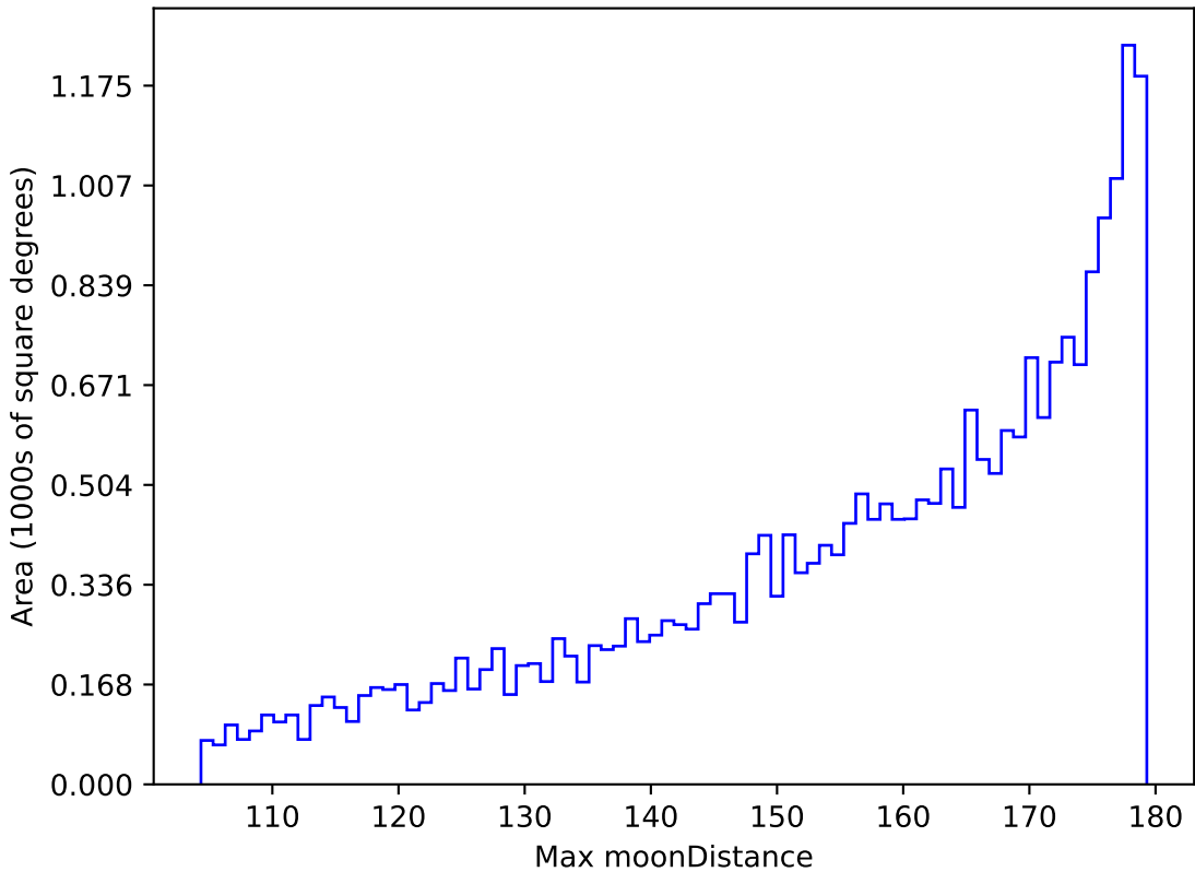
telescope_jerk_v3.5_10yrs All sky r band: Max moonDistance
