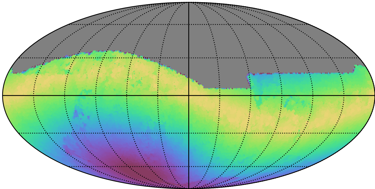
telescope_jerk_v3.5_10yrs All sky i band: Max moonDistance
