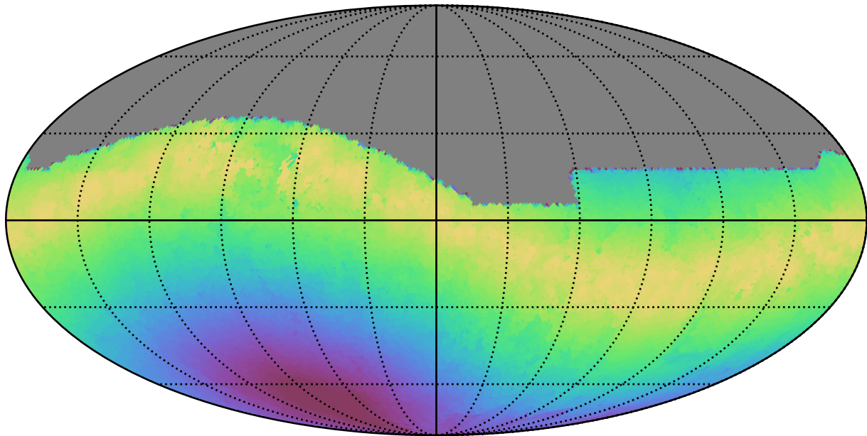
telescope_jerk_v3.5_10yrs All sky g band: Max moonDistance
