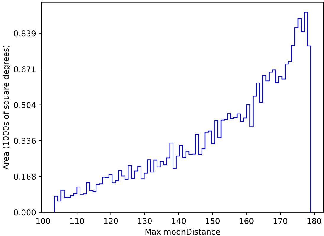
telescope_jerk_v3.5_10yrs All sky g band: Max moonDistance
