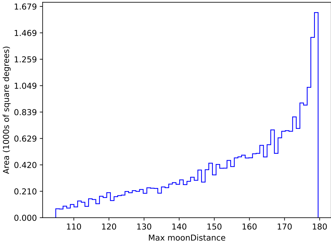
telescope_jerk_v3.5_10yrs All sky all bands: Max moonDistance
