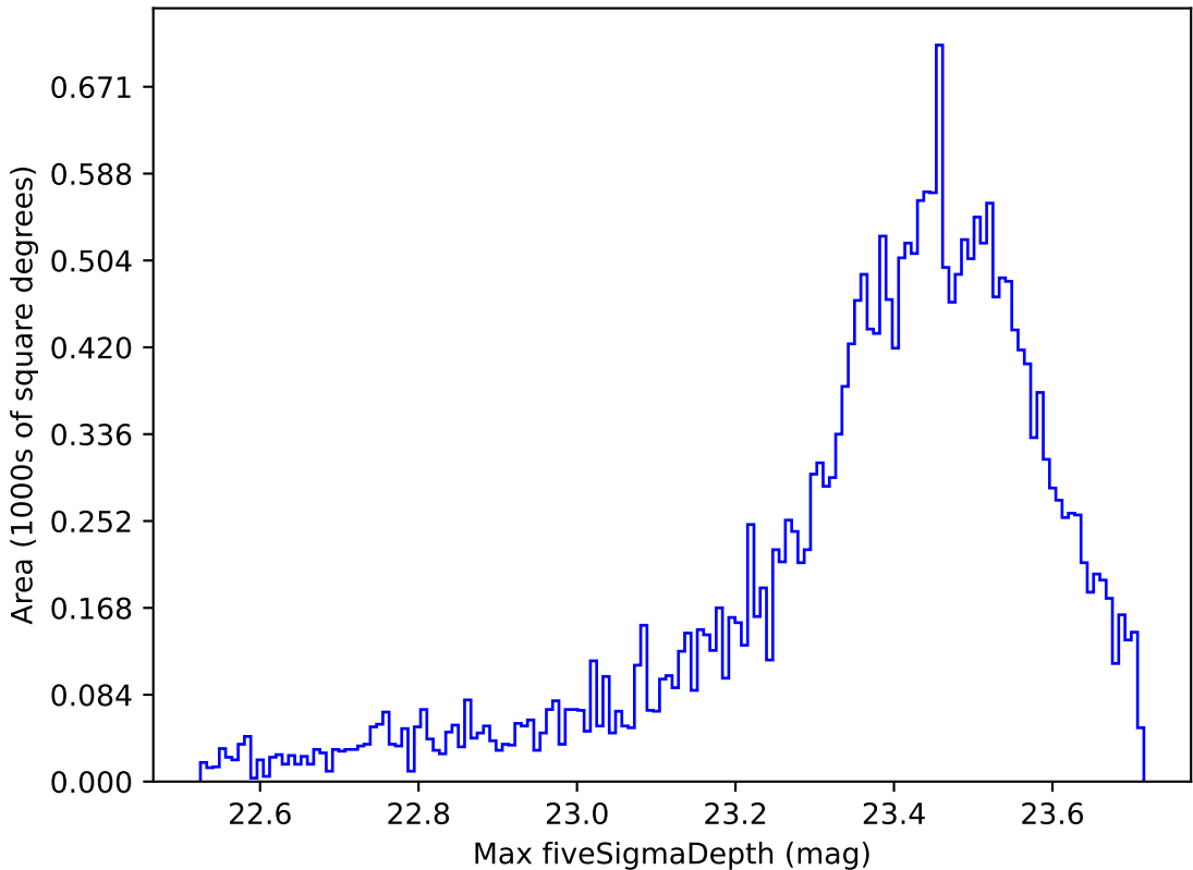
telescope_jerk_v3.5_10yrs Yr 1 z band: Max fiveSigmaDepth
