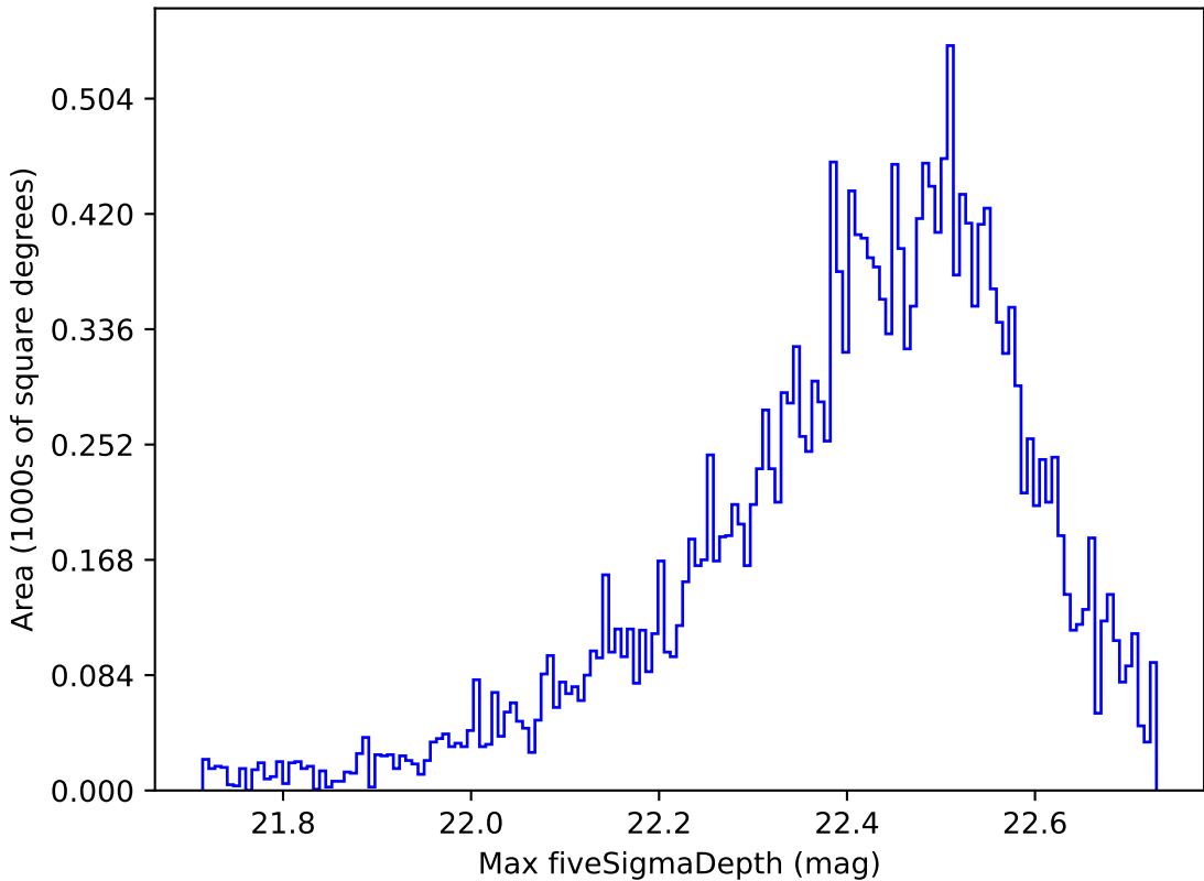
telescope_jerk_v3.5_10yrs Yr 1 y band: Max fiveSigmaDepth
