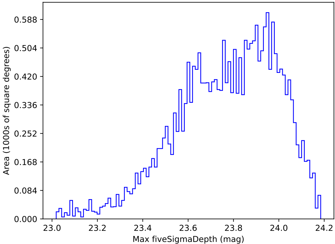
telescope_jerk_v3.5_10yrs Yr 1 u band: Max fiveSigmaDepth
