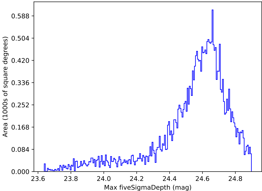
telescope_jerk_v3.5_10yrs Yr 1 r band: Max fiveSigmaDepth
