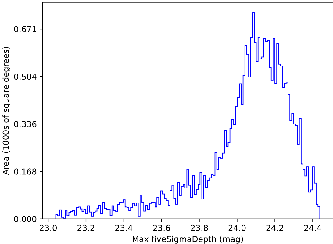
telescope_jerk_v3.5_10yrs Yr 1 i band: Max fiveSigmaDepth
