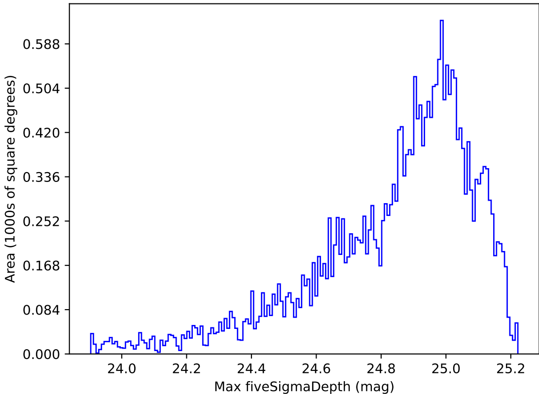
telescope_jerk_v3.5_10yrs Yr 1 g band: Max fiveSigmaDepth
