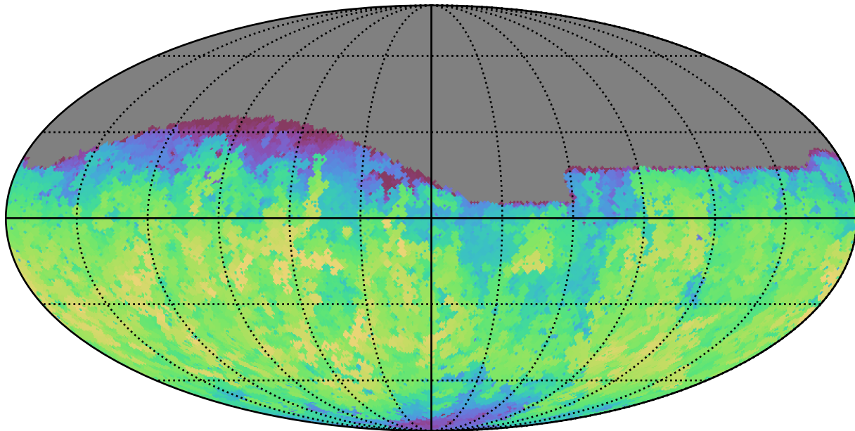
telescope_jerk_v3.5_10yrs Yr 1 all bands: Max fiveSigmaDepth
