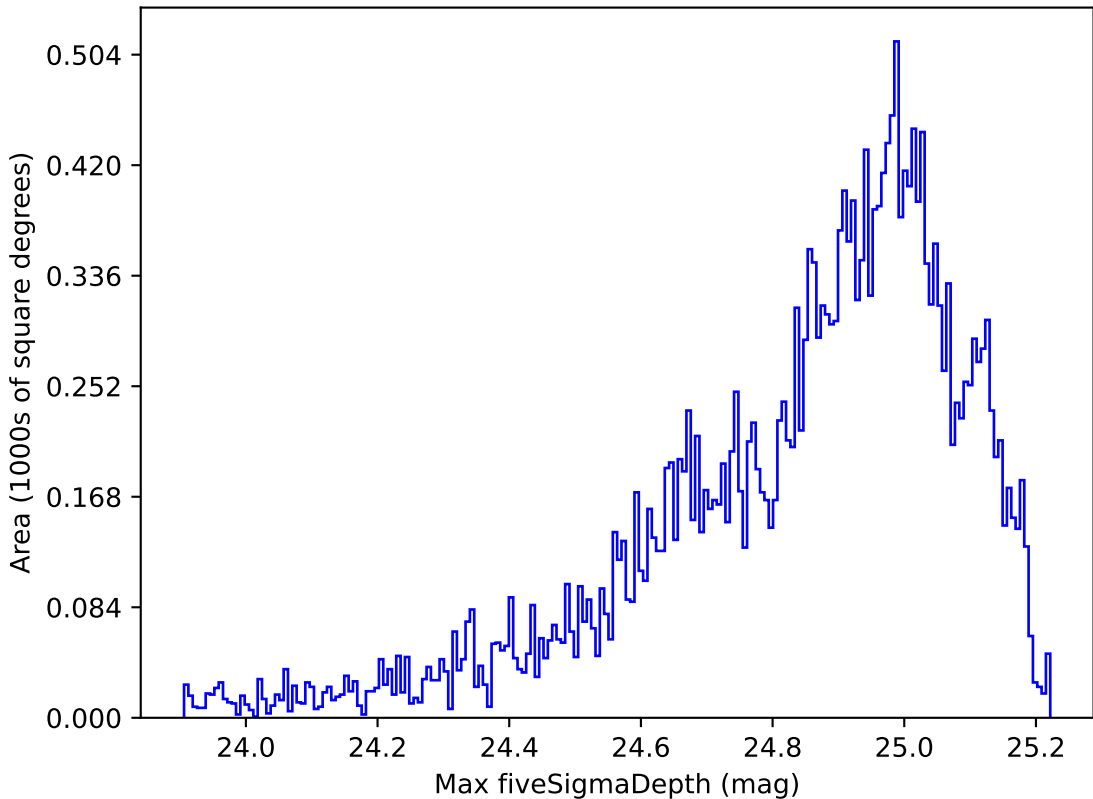
telescope_jerk_v3.5_10yrs Yr 1 all bands: Max fiveSigmaDepth
