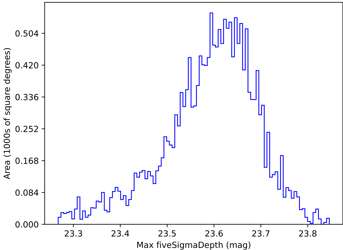
telescope_jerk_v3.5_10yrs WFD z band: Max fiveSigmaDepth
