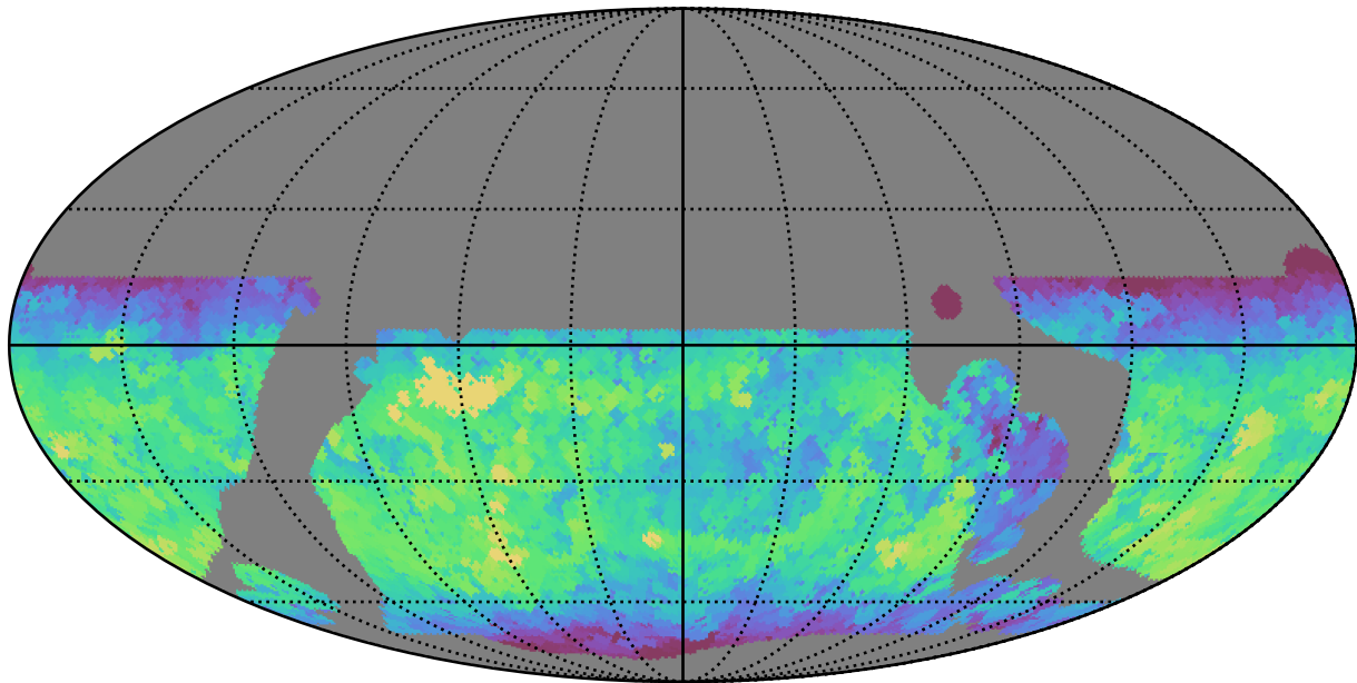
telescope_jerk_v3.5_10yrs WFD y band: Max fiveSigmaDepth
