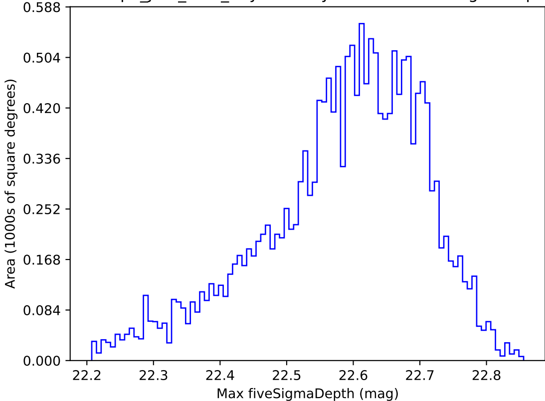
telescope_jerk_v3.5_10yrs WFD y band: Max fiveSigmaDepth
