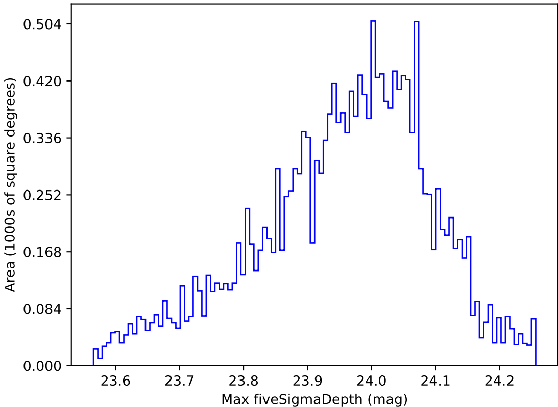
telescope_jerk_v3.5_10yrs WFD u band: Max fiveSigmaDepth
