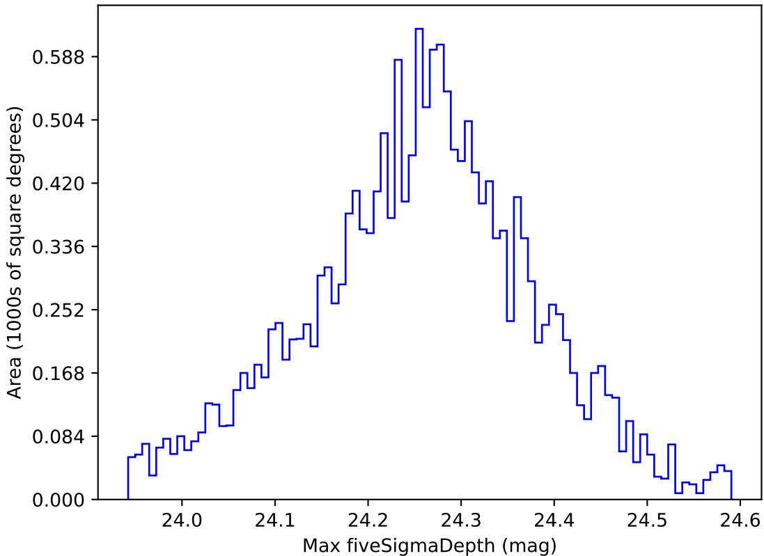
telescope_jerk_v3.5_10yrs WFD i band: Max fiveSigmaDepth
