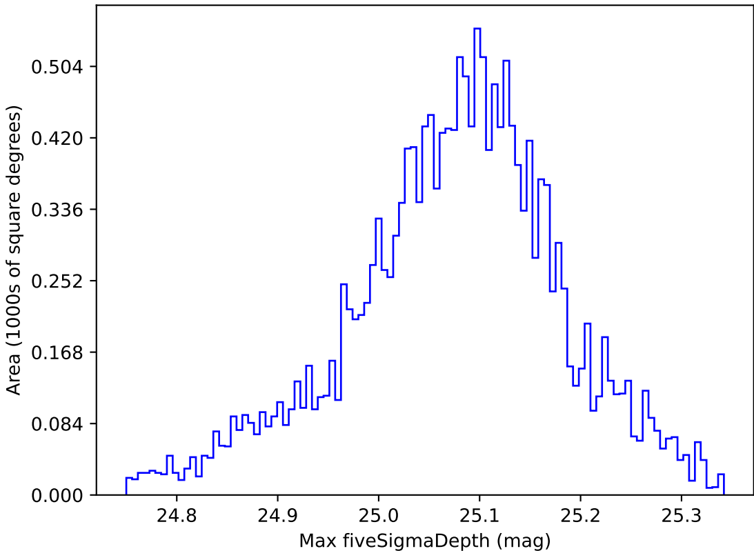
telescope_jerk_v3.5_10yrs WFD g band: Max fiveSigmaDepth
