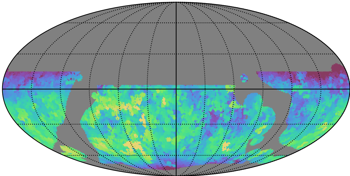
telescope_jerk_v3.5_10yrs WFD all bands: Max fiveSigmaDepth
